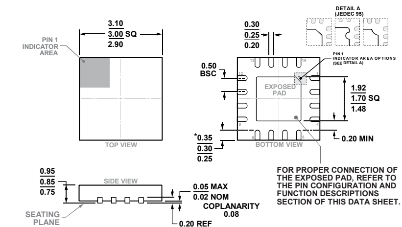
Figure 26. 16-Lead Lead Frame Chip Scale Package [LFCSP] 3 mm × 3 mm Body and 0.85 mm Package Height (CP-16-38)
