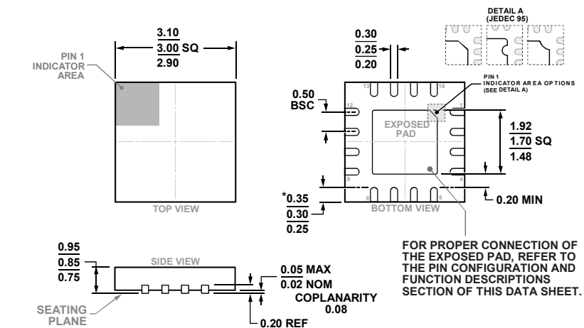
Figure 26. 16-Lead Lead Frame Chip Scale Package [LFCSP] 3 mm x 3 mm Body and 0.85 mm Package Height (CP-16-38)
