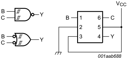
Fig 5. 2-input NAND gate or 2-input OR with both inputs inverted
