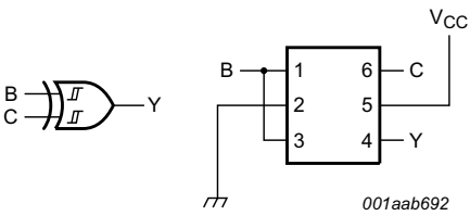
Fig 9. 2-input XOR gate
