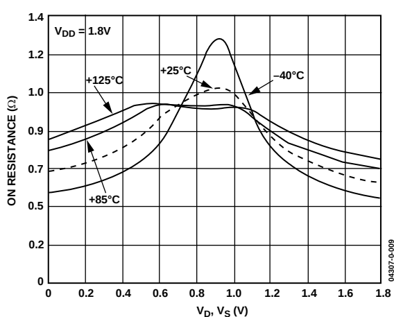
Figure 8. On Resistance vs. V_D ( V_S ) for Different Temperature, V_{DD} = 1.8 V
