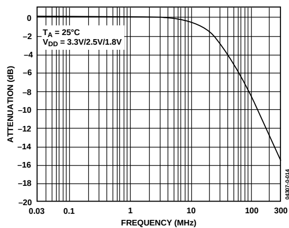
Figure 14. Bandwidth
