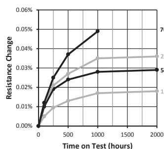
Biased Damp Heat Stability
