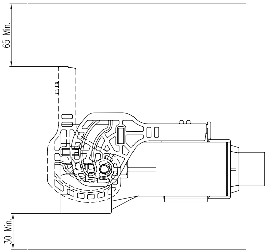
REVERSE LEVER
