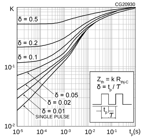
Figure 3: Thermal impedance
