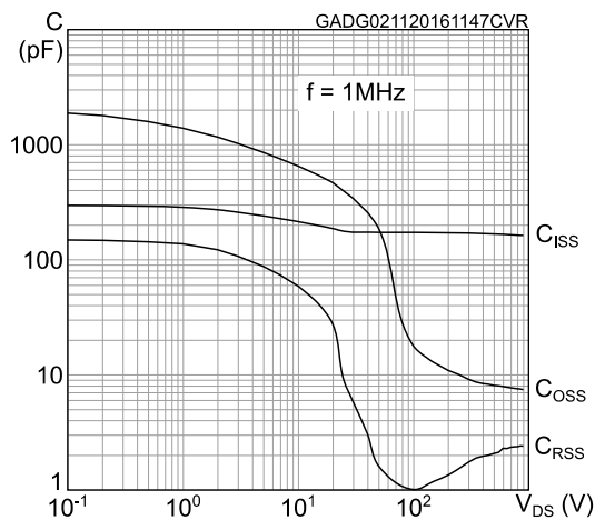
Figure 8: Capacitance variations
