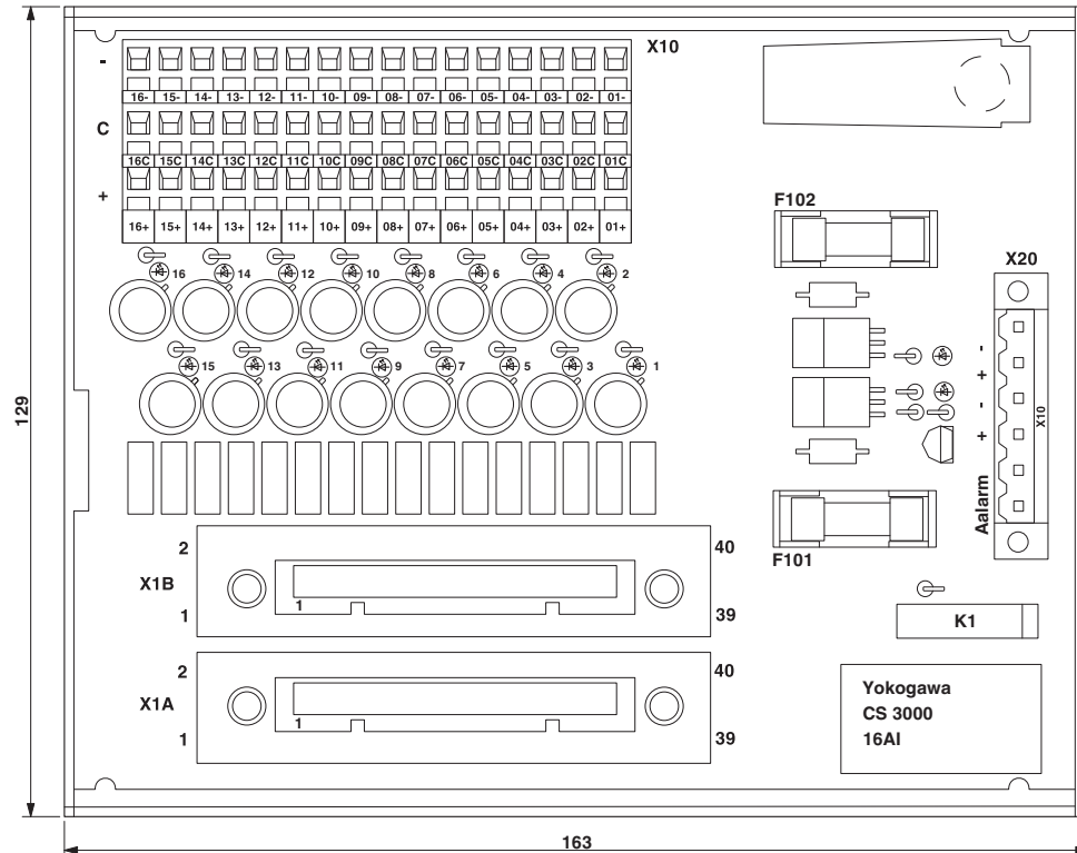
Dimensional drawing
