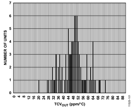
Figure 7. TCV_{OUT} Distribution, -40^{\circ}\text{C} to +210^{\circ}\text{C} , FLATPACK Package
