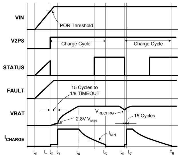
FIGURE 19. OPERATION WAVEFORMS
