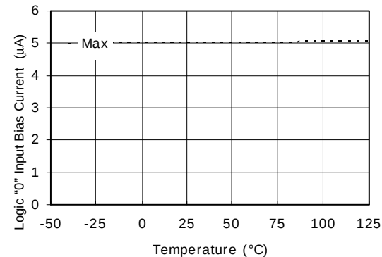
Figure 17A. Logic "0" Input Bias Current vs. Temperature
