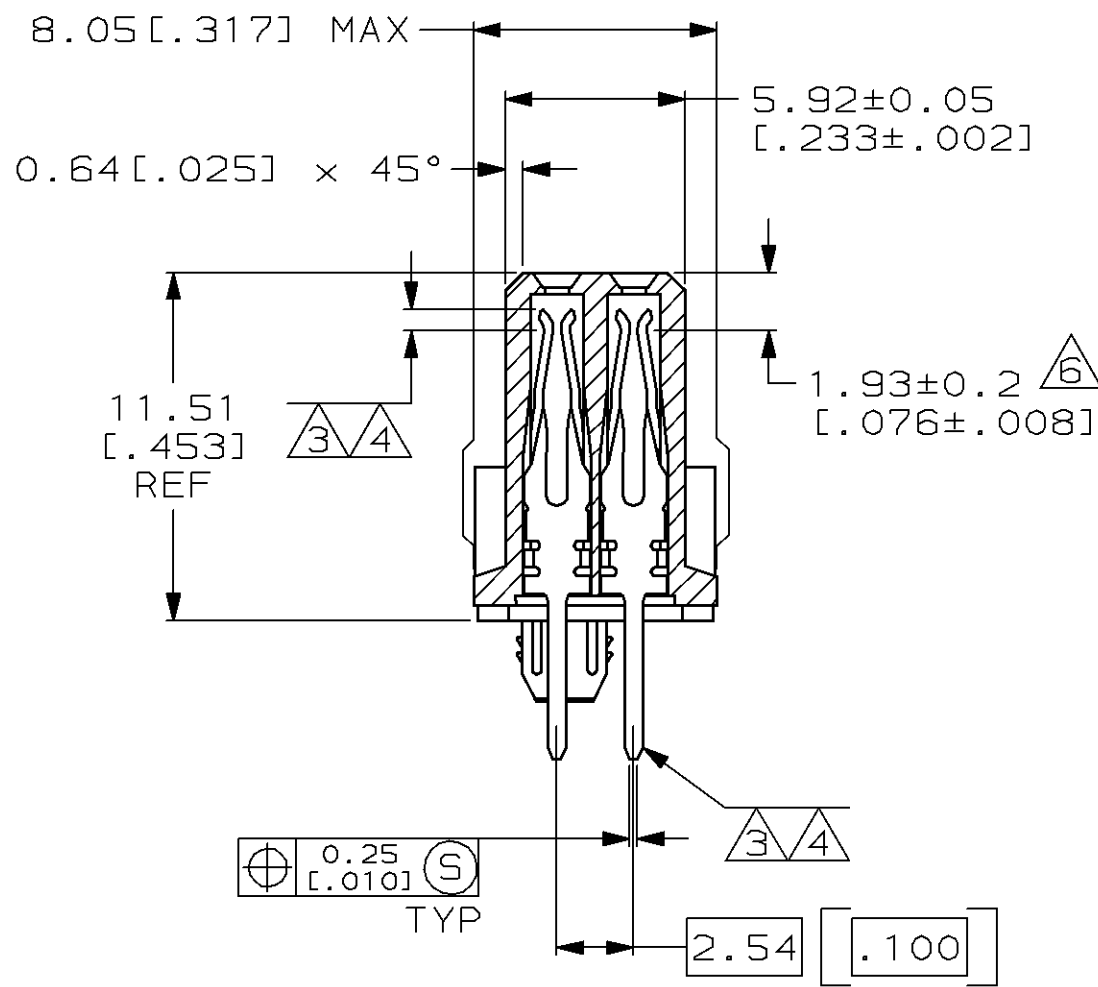
SECTION X-X
