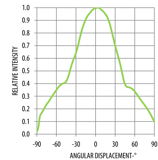
Figure 5: Radiation Pattern
