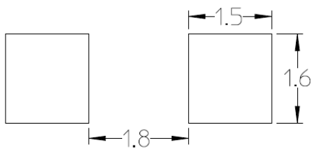
Figure 11: Recommended Solder Pad (Units: mm)
