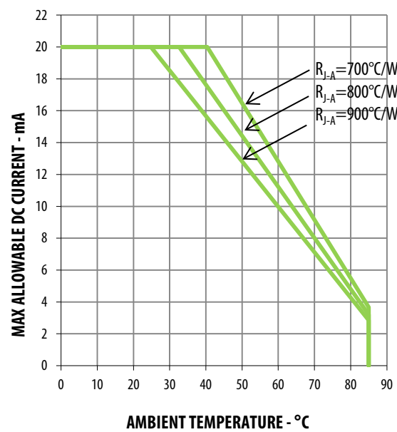
Figure 10: Derating Curve
