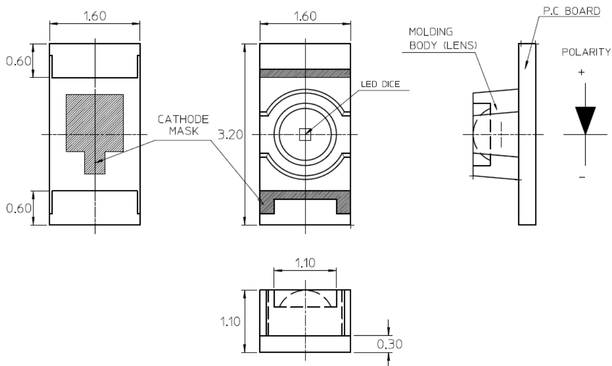
Figure 1: Package Dimensions
