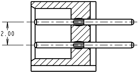
SECTION X-X
