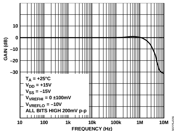
Figure 25. Small-Signal Response
