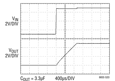
5V Start-Up Response with a 3.3μF Output Capacitor
