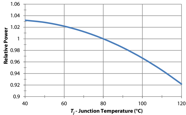
Forward Voltage vs T_j : Normalized to I_f = 6 A and T_j = 80^\circ\text{C} 405 nm
