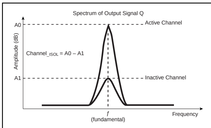
Channel Isolation
