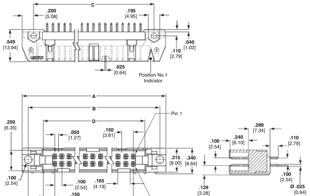
Right-Angle PCB Mount
