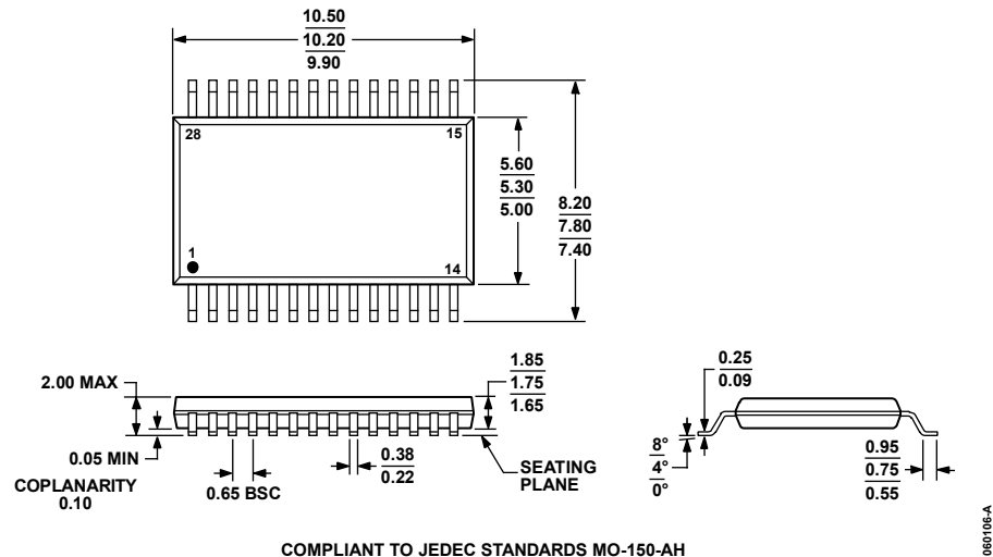
Figure 13. 28-Lead Shrink Small Outline Package [SSOP] (RS-28) Dimensions shown in millimeters
