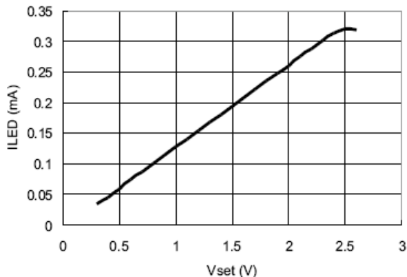
11. I_{LED} VS V_{SET} ( V_{IN}=16\text{V} , 3 LEDs, 47\mu\text{H} , R_s=0.15\Omega )
