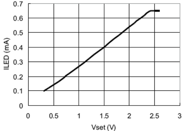
12. I_{LED} VS V_{SET} ( V_{IN}=16\text{V} , 3 LEDs, 100\mu\text{H} , R_s=0.3\Omega )
