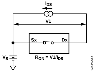
Figure 14. On Resistance
