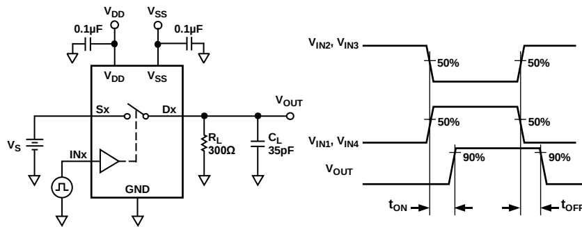
Figure 17. Switching Times
