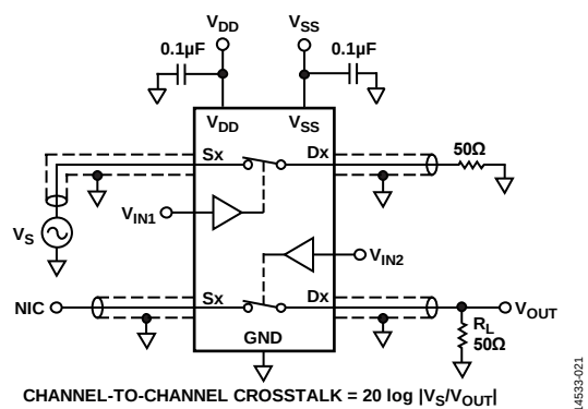
Figure 21. Channel-to-Channel Crosstalk
