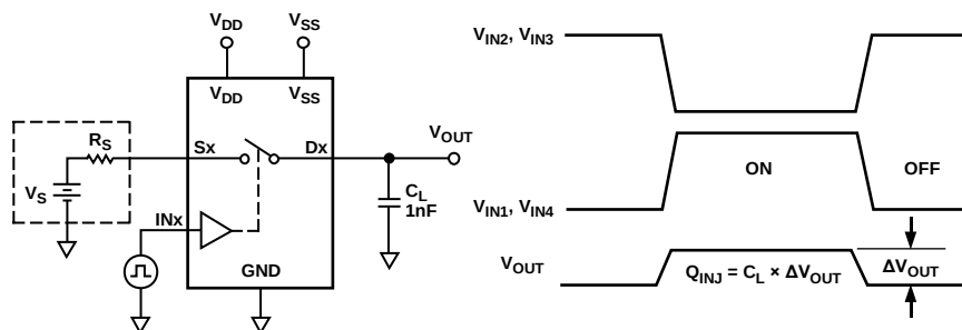
Figure 19. Charge Injection
