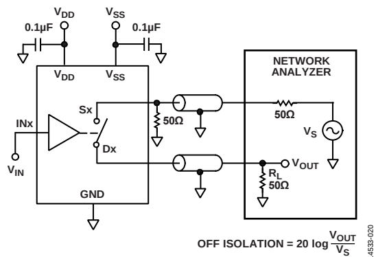
Figure 20. Off Isolation
