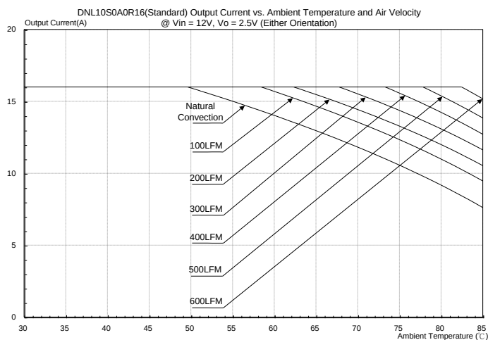
Figure 33: DNL10S0A0R16(Standard) Output current vs. ambient temperature and air velocity @ Vin=12V,
