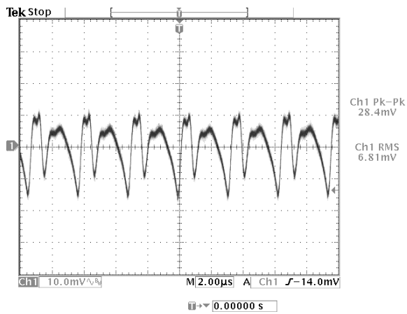
Figure 8: Output ripple & noise at 12Vin, 2.5V/16A out
