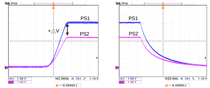
Figure 29: Ratio-metric
