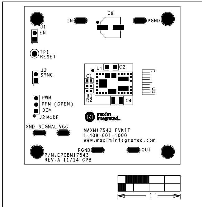
Figure 1. MAXM17543 EV Kit Component Placement Guide— Component-Side
