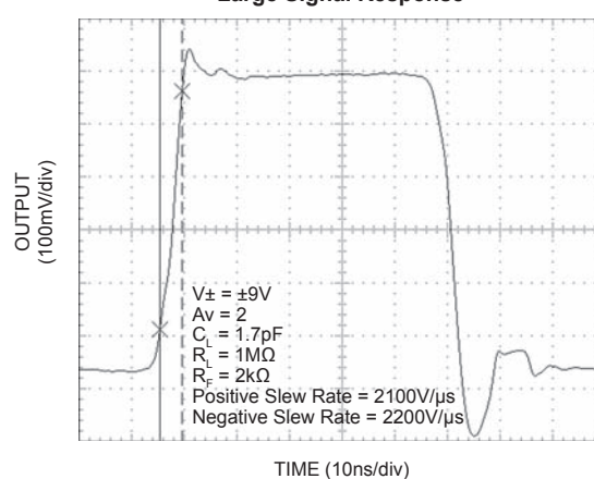
Large Signal Response
