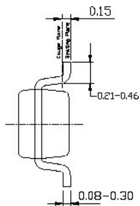
END VIEW
