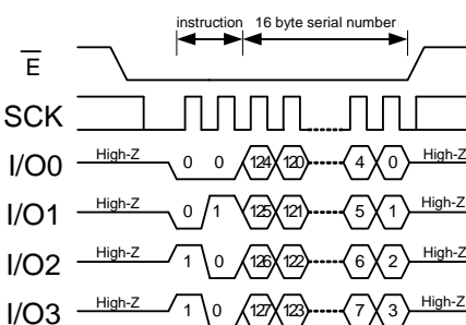
WRSNR in SPI Mode
