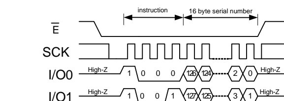
WRSNR in DPI Mode
