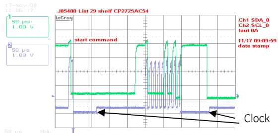
Figure 14. Example waveforms showing clock stretch
