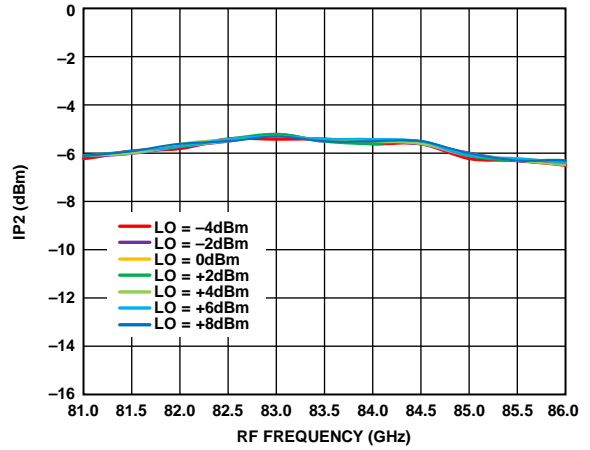
Figure 77. Input IP2 vs. RF Frequency at Various LO Powers, IFIN = 5 dBm, IF = 2000 MHz, LSB
