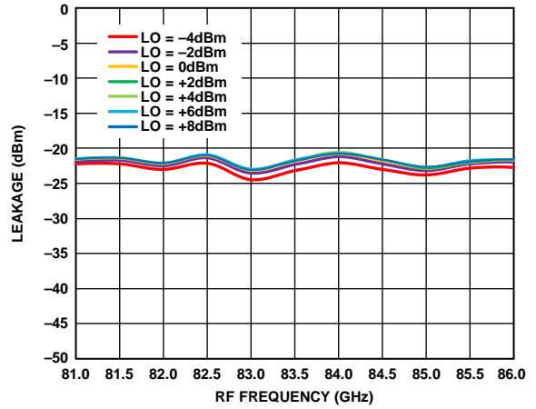
Figure 78. 6x LO Leakage at RFOUT vs. RF Frequency at Various LO Powers, IFIN = 5 dBm, IF = 2000 MHz, LSB
