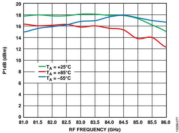
Figure 76. Input P1dB vs. RF Frequency at Various Temperatures, LO = 2 dBm, IF = 2000 MHz, LSB
