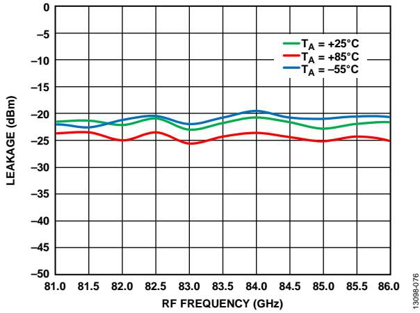
Figure 75. 6x LO Leakage at RFOUT vs. RF Frequency at Various Temperatures, IFIN = 5 dBm, IF = 2000 MHz, LSB
