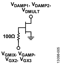
Figure 5. V GMIX , V DAMP1 , V DAMP2 , V DMULT , V VGAMP , V VGX2 , V VGX3 Interface
