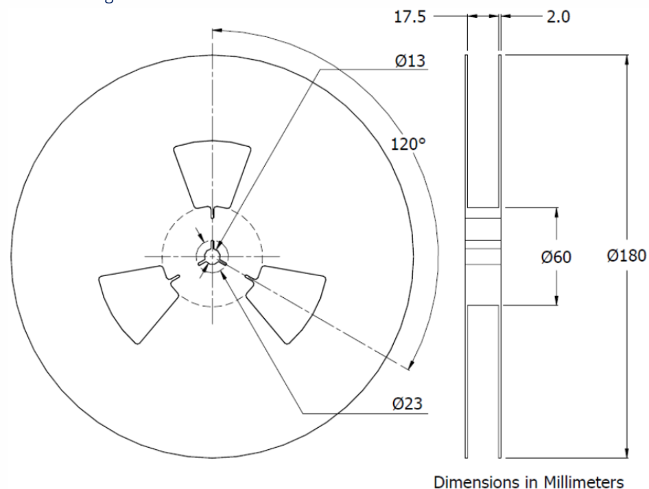
Reel Drawing
