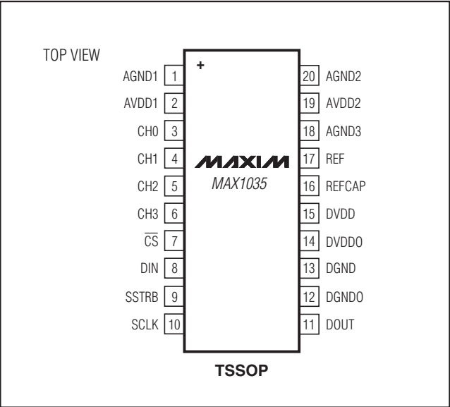
Pin Configurations (continued)
