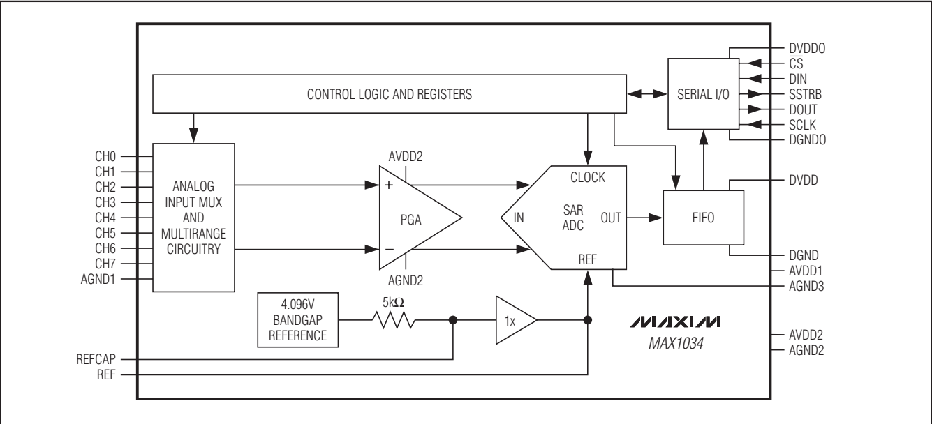
Block Diagram
