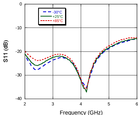
Antenna Ports Return Loss
