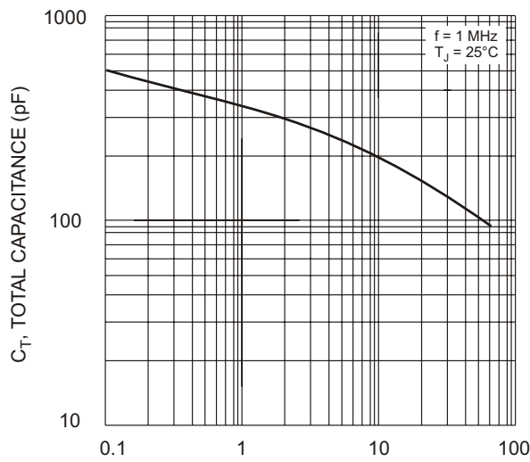
Fig. 5 Typical Capacitance
