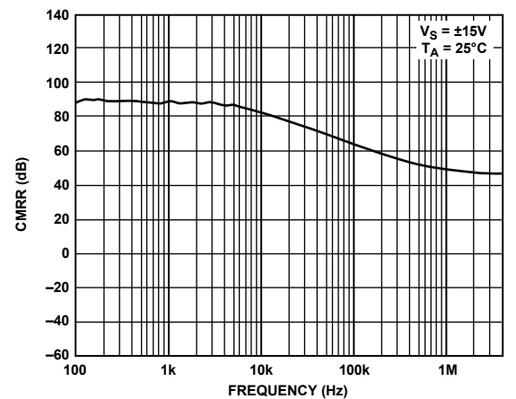
Figure 19. AD8682 CMRR vs. Frequency
