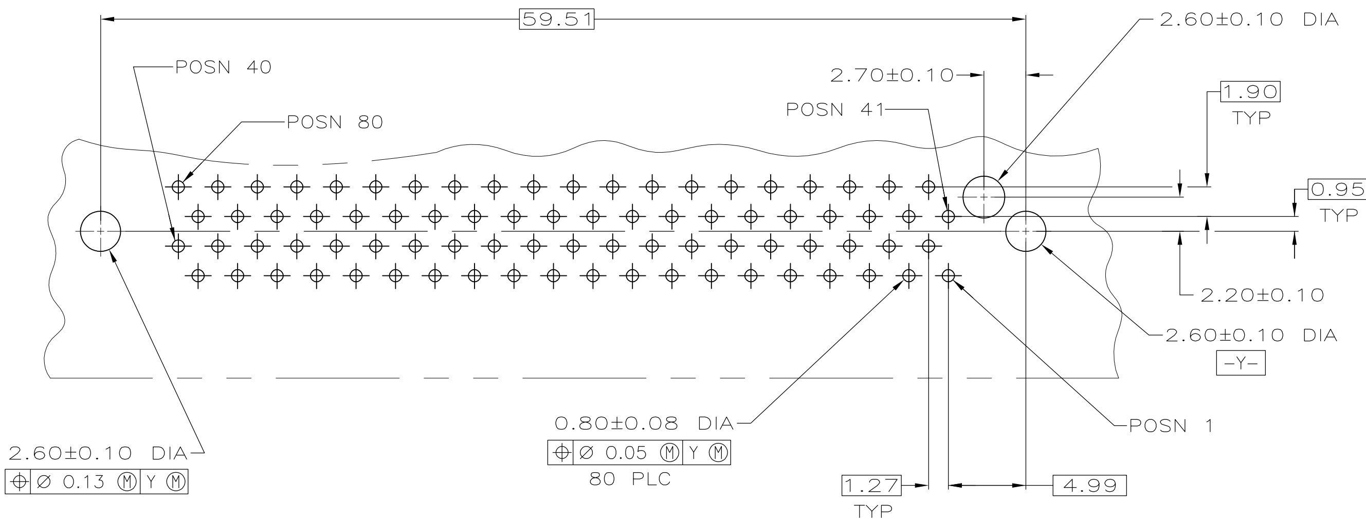
SUPERCEDED BY 787311-5 OBSELETE 8 9 4.57 80 787311-5 8 9 3.18 80 787311-4 2 3 4.57 80 787311-3 OBSELETE 2 3 3.18 80 787311-2 OBSELETE 2 3 3.18 80 787311-1 FINISH J POSN PART NUMBER
