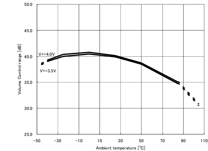
Volume control range vs ambient temperature ( VLC=0Ω/100kΩ )
