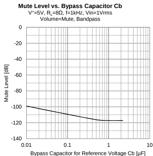
Fig. 13 Mute Level vs. C_b
