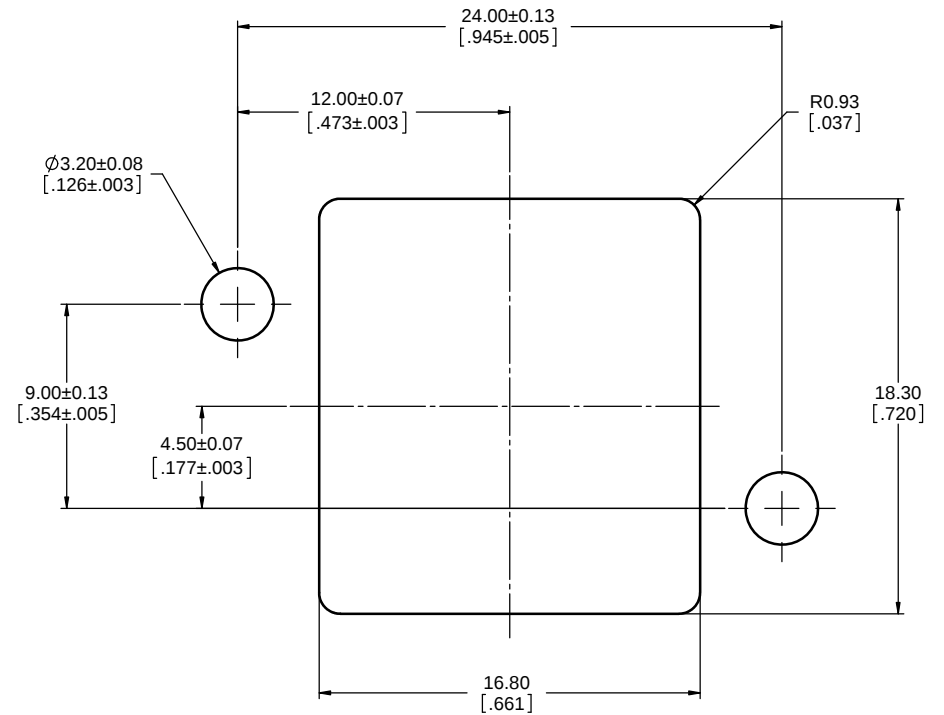
RECOMMENDED PANEL CUTOUT OUTSIDE VIEW OF PANEL
