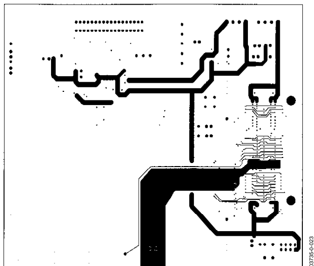
Figure 25. Power Plane 1
