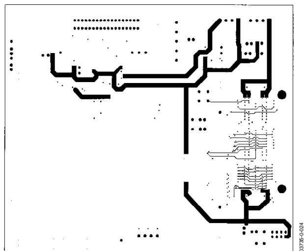
Figure 26. Power Plane 2
