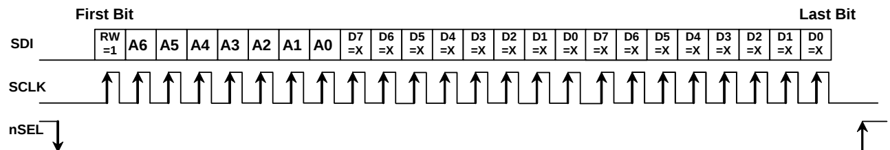
Figure 3. SPI Timing—Burst Write Mode
