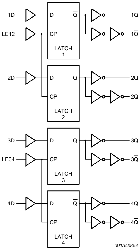
Fig 4. Logic diagram
