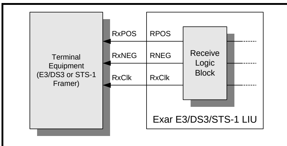
FIGURE 28. THE TYPICAL INTERFACE FOR THE TRANSMISSION OF DATA IN A DUAL-RAIL FORMAT, FROM THE RECEIVE SECTION OF THE XRT73LC03A TO THE RECEIVING TERMINAL EQUIPMENT
