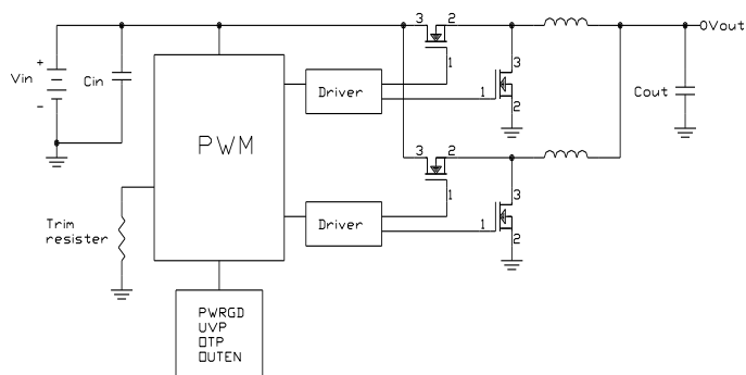
Figure 25: Block Diagram
