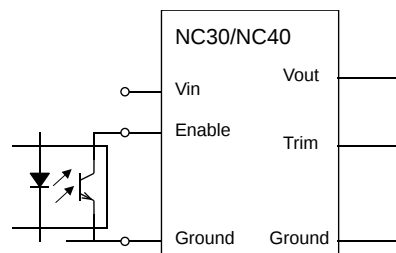
Figure 28: Enable input drive circuit example with isolation.
