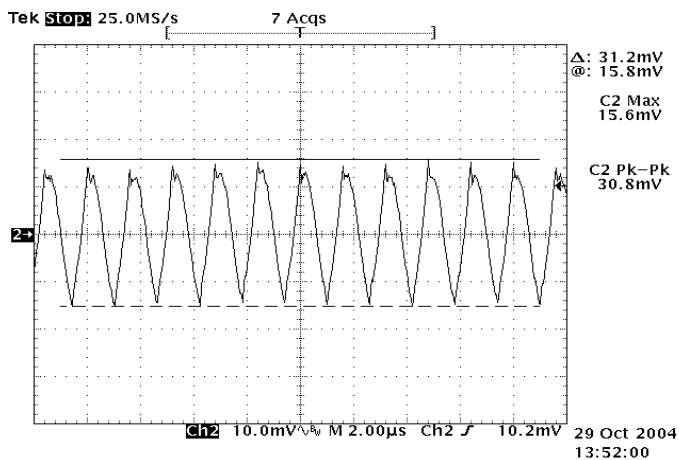
Figure 11: Output ripple & noise at 12Vin, 1.8V/40A out
