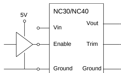
Figure 27: Enable input drive circuit using logic gate.
