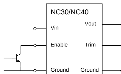
Figure 26: Enable Input drive circuit for NC series
