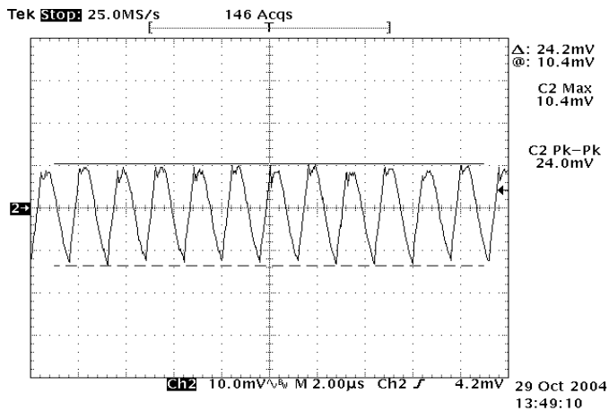
Figure 9: Output ripple & noise at 12Vin, 1.2V/40A out
