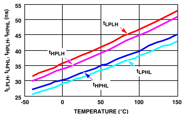
FIGURE 15. ISL2110 PROPAGATION DELAYS vs TEMPERATURE
