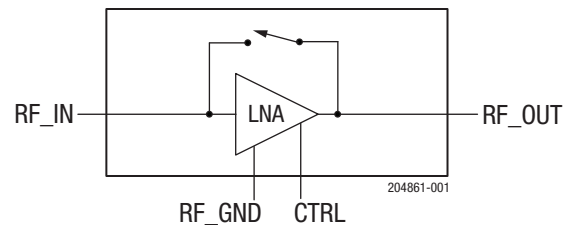
Figure 1. SKY65803-696LF Block Diagram
