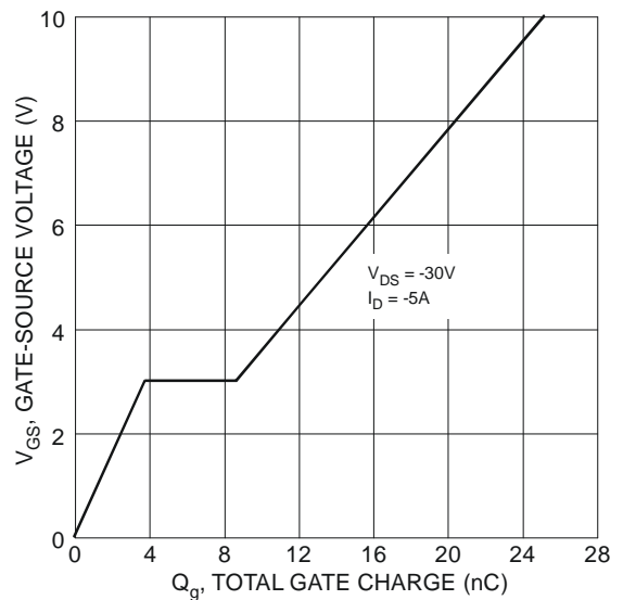
Figure 12 Gate-Charge Characteristics
