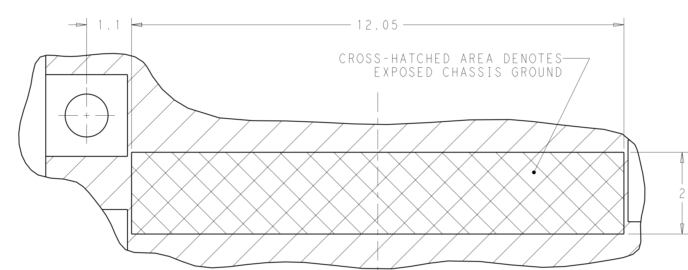
DETAIL J RECOMMENDED PT CONNECTOR LAYOUT SCALE 12:1
