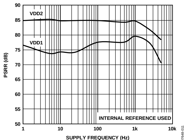
Figure 38. PSRR vs. Supply Frequency (350 mV p-p Ripple on VDD2, 600 mV Ripple on VDD1)
