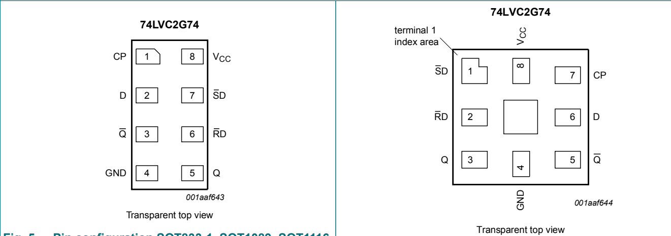
Fig. 5. Pin configuration SOT833-1, SOT1089, SOT1116 and SOT1203 (XSON8)
