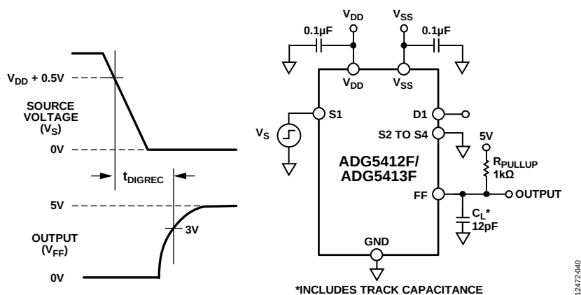
Figure 45. Interrupt Flag Recovery Time, t_{DIGREC} , with a 1 kΩ Pull-Up Resistor
